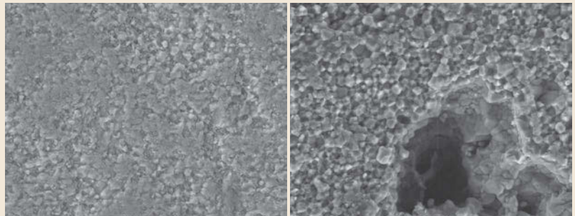
500x. The density of the grain, however, is tighter in the black Arkansas stone (left).
