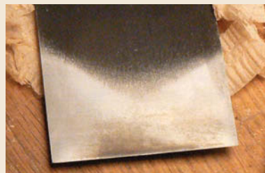
Flat back. The back is the most important surface to address when sharpening an edge tool. Notice the wear bevel at the cutting edge.
