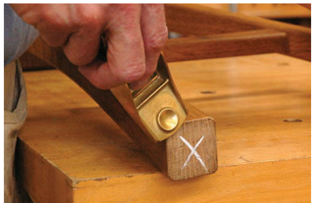
There's got to be a better way. Truing legs with a block plane requires time and ingenuity to make sure the piece stays stable and doesn't tear out as you attempt to trim it to length.
