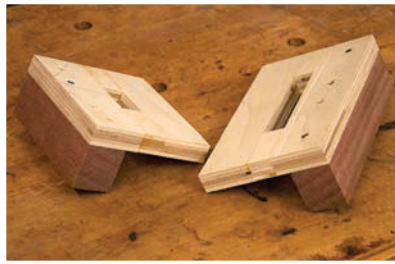
Mortises on demand. These jigs, combined with router guide bushings, ensure consistent-sized mortises in multiple locations.
