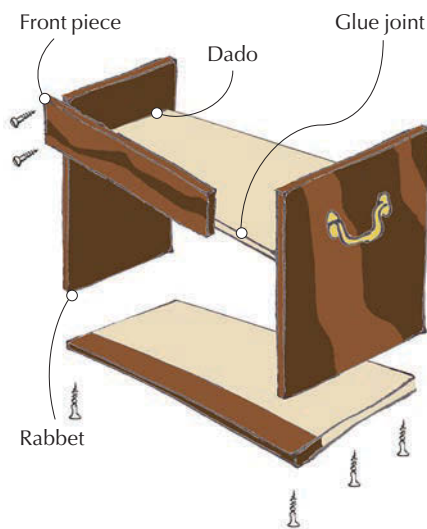
Carcase. The basic carcass is glued and screwed together. The bottom and back are let into rabbets. The front is applied, but this necessitates filler strips on edges of the sides to maintain a flat front.
