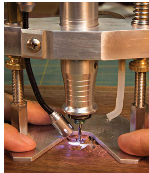
Rout out the waste. A trim router, Dremel or carving tool attached to a plunge base routs out the bulk of the waste in the cavity.
