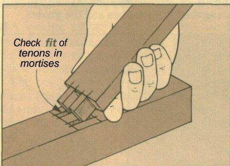
Trimming to fit. After both tenons have been rough-cut, test the fit in the twin mortises. The cheeks and shoulders will probably have to be shaved for a perfect fit.
