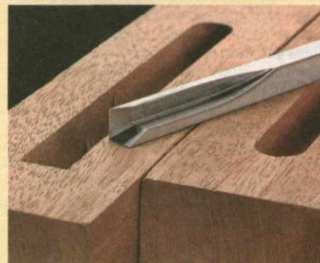
A Square ends. Like driving a square peg in a round hole, this corner chisel squares up the rounded ends of a mortise.
