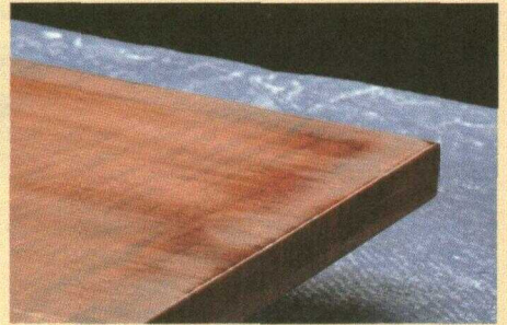
Low spots. After wet-sanding, high spots in the finish show up as dull areas. Sand until the low shiny areas become dull too.
