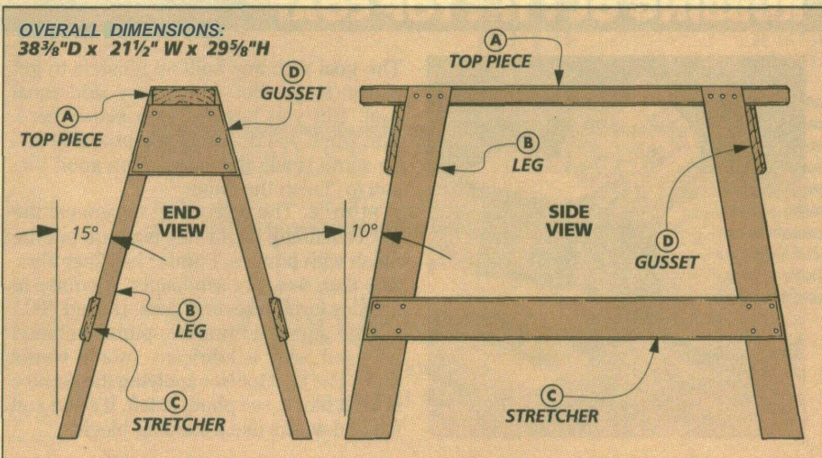
A The notches cut in the top piece angle the legs outward in two directions. Gussets and stretchers brace the legs to make the sawhorse strong and sturdy.
