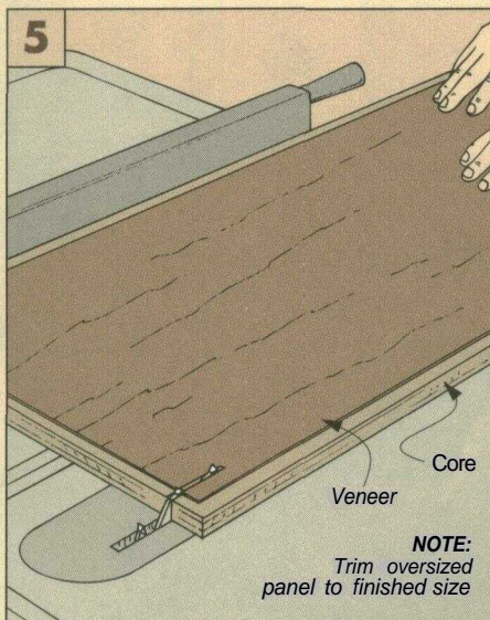
Cut to size. Cut the core and veneer to size on the table saw. A fine tooth blade reduces chipout—especially on crosscuts.
