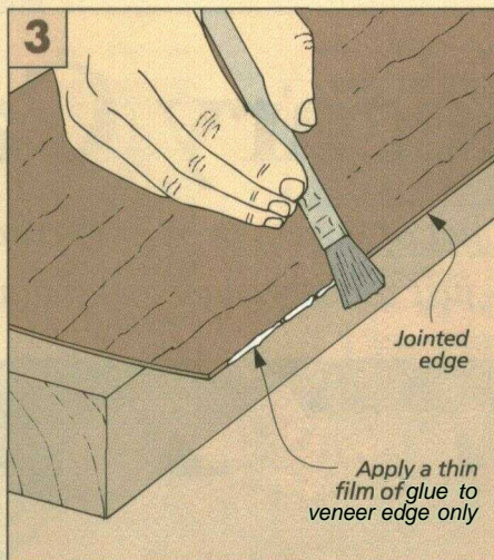
Edge gluing veneer. Use a brush to spread a thin film of glue along the jointed edges to hold the veneer pieces together.
