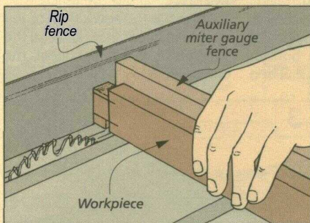
Outside cheeks. All cuts for the twin tenons can be made on the table saw. An auxiliary fence on the miter gauge prevents chipout on the back side of the cut.
