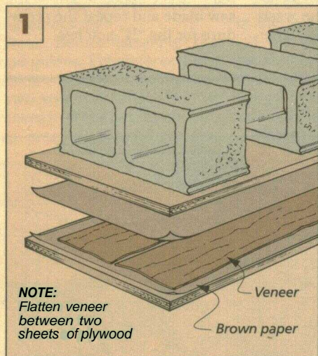
Flattening veneer. Pressing the veneer between two weighted sheets of plywood will usually flatten the veneer overnight.
