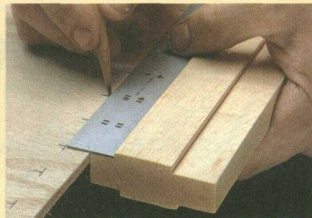
A lay-out tool helps when marking many screw holes all inset the same distance. It can be used to mark four different-size insets.
