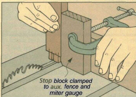
Inside cheeks. The inside cheeks of the tenons are cut with the workpiece standing on end. A stop block clamped to the auxiliary fence helps support the workpiece.
