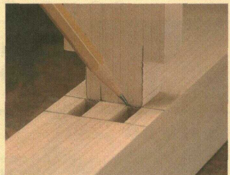
Mark tenons from mortises. The mortises on the leg can be used to quickly indicate the position of the tenons on the rail.
