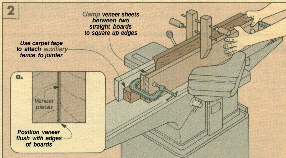
Square up the edges. Square edges are needed to join veneer pieces for an invisible seam. Run the scrap boards with ve-
