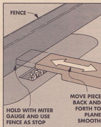
3 To remove the V-cuts, slide the workpiece right and left over blade while pushing it forward and back.
