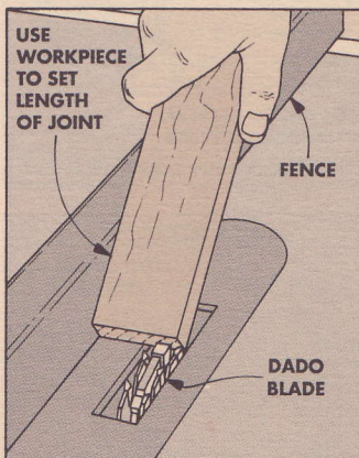
1 Mount a dado blade and set the fence as a stop. Use a workpiece to set the distance between the fence and blade.
