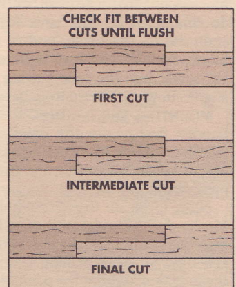
4 Make repeated passes over the end of two test pieces. Then check the fit until the outside surfaces are flush.
