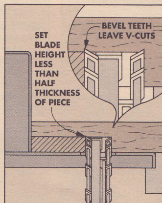
2 When a dado set is used, the bevel teeth on the outside blades make small V-cuts in the face of the half lap.
