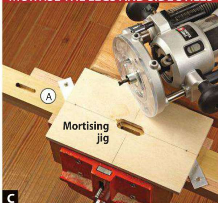
C Precisely mark the centerlines of the mortises and center the mortising jig on the lines. Clamp the jig in place; then, rout the mortises.
