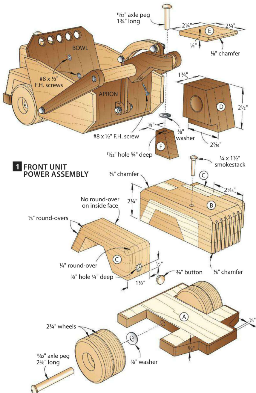
B Apply glue to the inside face of each front fender (C) and align the edges of the wheel well on the fender and the chassis (A).
