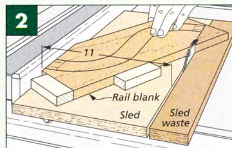
Reverse. Now reset the fence to the position shown in the drawing and flip the sled to cut off the opposite corner.
