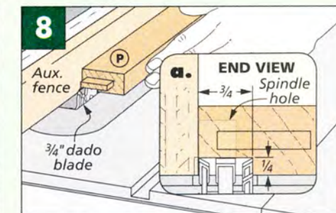
Rabbet. By cutting a rabbet on the back face of the bottom rail, you open up the mortises, so you can slide in the balusters.
