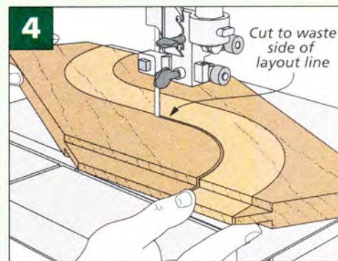
Curve. After laying out the shape using the template, cut the curved shape at the band saw, staying on the waste side of the cut.
