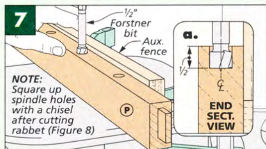
Mortises. Cut the mortises in the bottom rail by drilling out the waste first. Square the corners after cutting the rabbet and exposing the holes.
