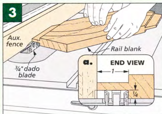
Tenons. With a dado blade installed, cut the tenon cheeks on the blank. Raise the blade slowly to sneak up on a snug-fitting tenon.
