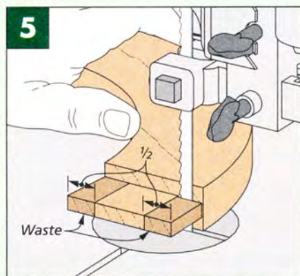
Shoulders. The band saw is also the perfect tool for cutting away the waste from the shoulders of the tenon.
