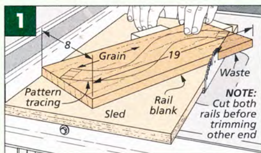
Sled. Using the sled described on page 33, set the rip fence so the edge of the sled contacts the blade and cut the first corner of both blanks.
