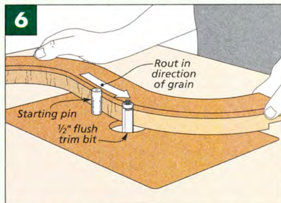
Trimming. To rout with the grain on both ends of the curved rail, you'll need to attach the template to the opposite face after routing the first curve.
