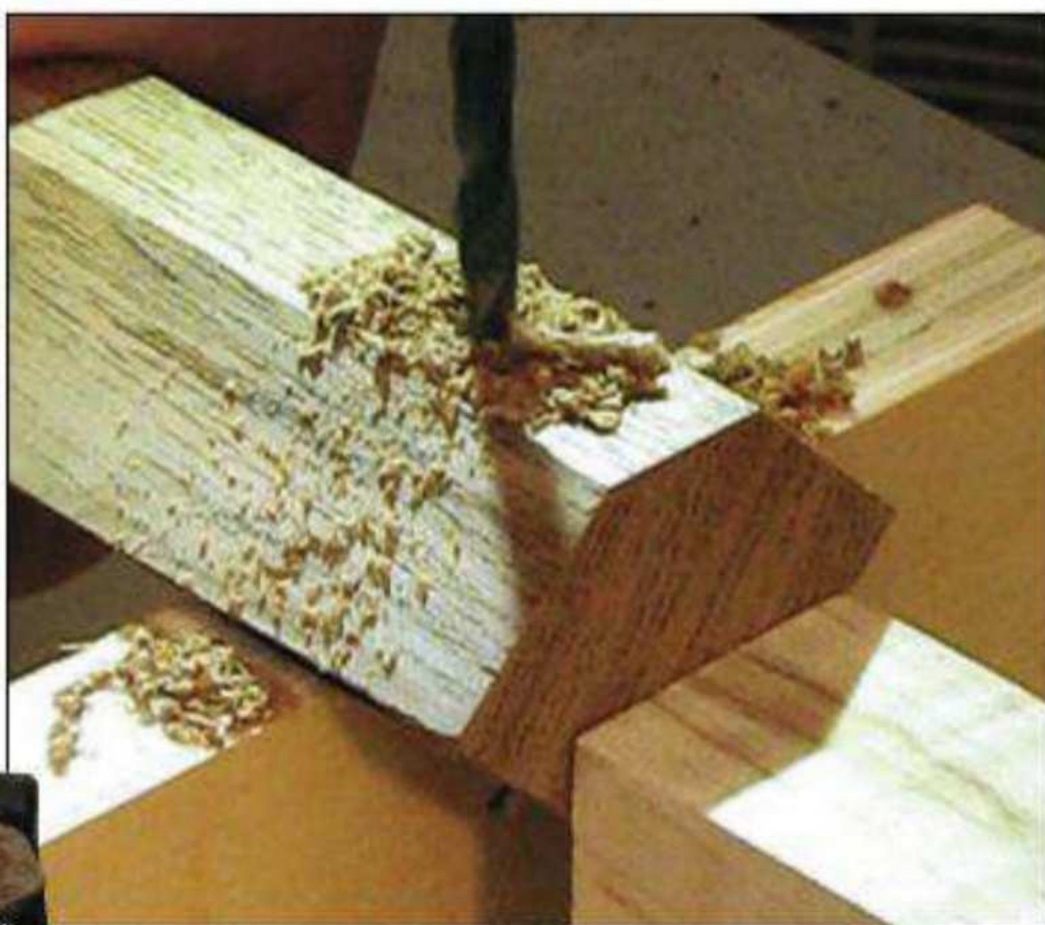
A shop-made cradle jig with a registration stop will help to ensure that the screws and countersinks are perfectly positioned and drilled.
