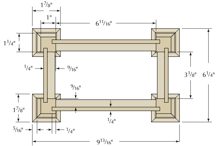
CARCASE PLAN
