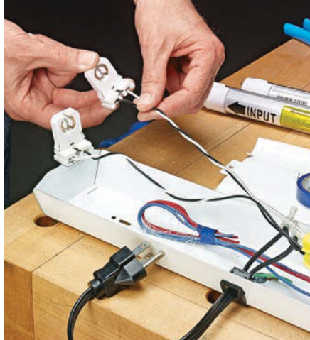
▲ At one end of the fixture, connect the wires from the new tombstones to the power source to supply the LED tubes.
