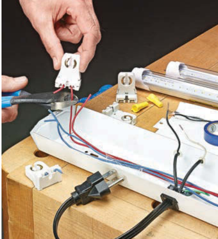
▲ To replace fluorescent tubes, start by cutting the power wires and the wires to the old tombstone sockets, then remove
